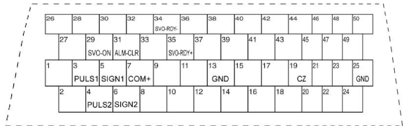
KSDG (50 Pins)
